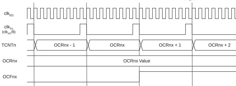
Figure 15-10. Timer/Counter Timing Diagram, Setting of OCF0x, with Prescaler ( f_{\text{clk}_{I/O}}/8 )
