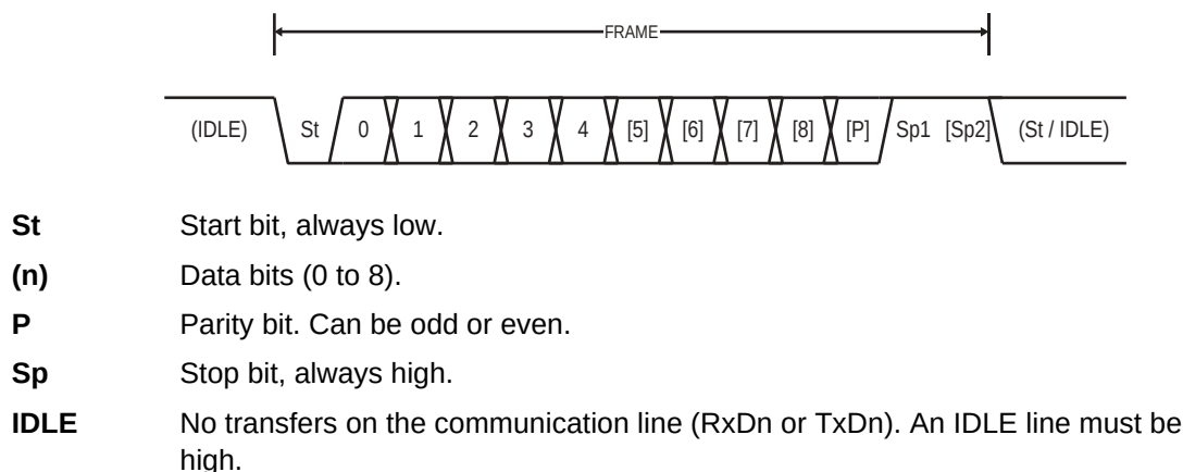
Figure 20-4. Frame Formats
